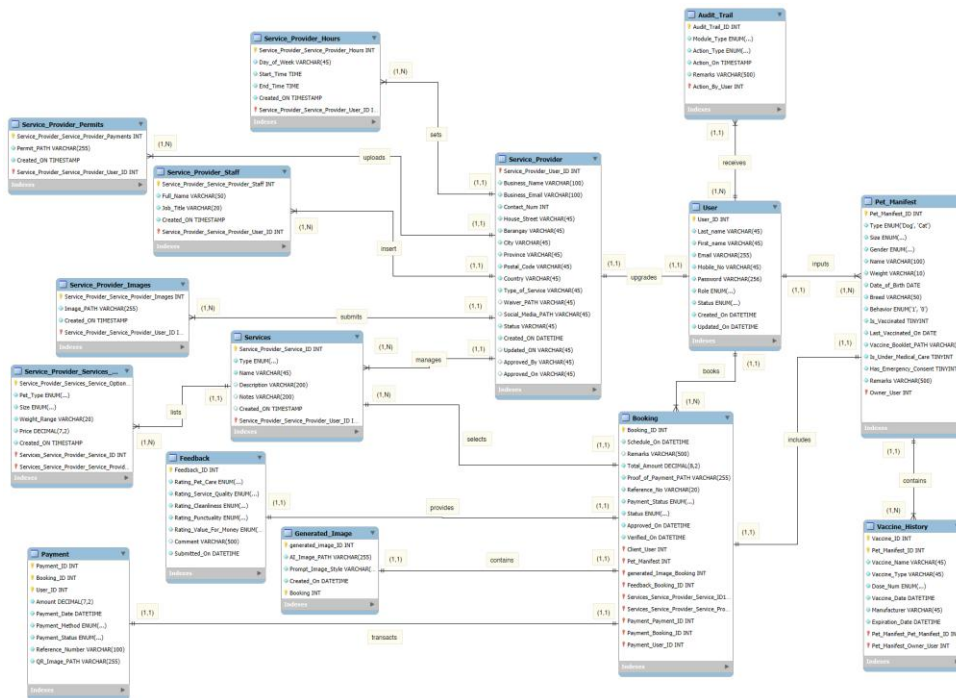
Figure 3 furlink ERD
